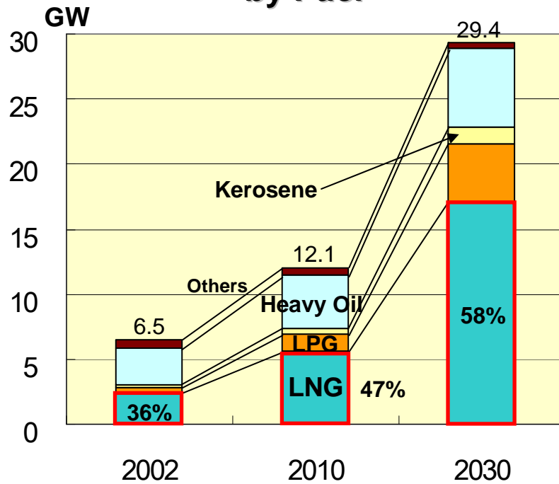
Distributed Power Generation Capacity by Fuel
