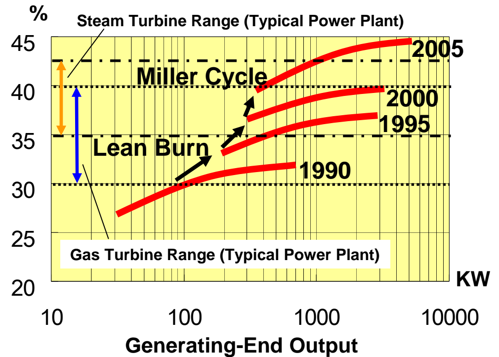
Power Generation Efficiency (LHV) On Gas Engine
