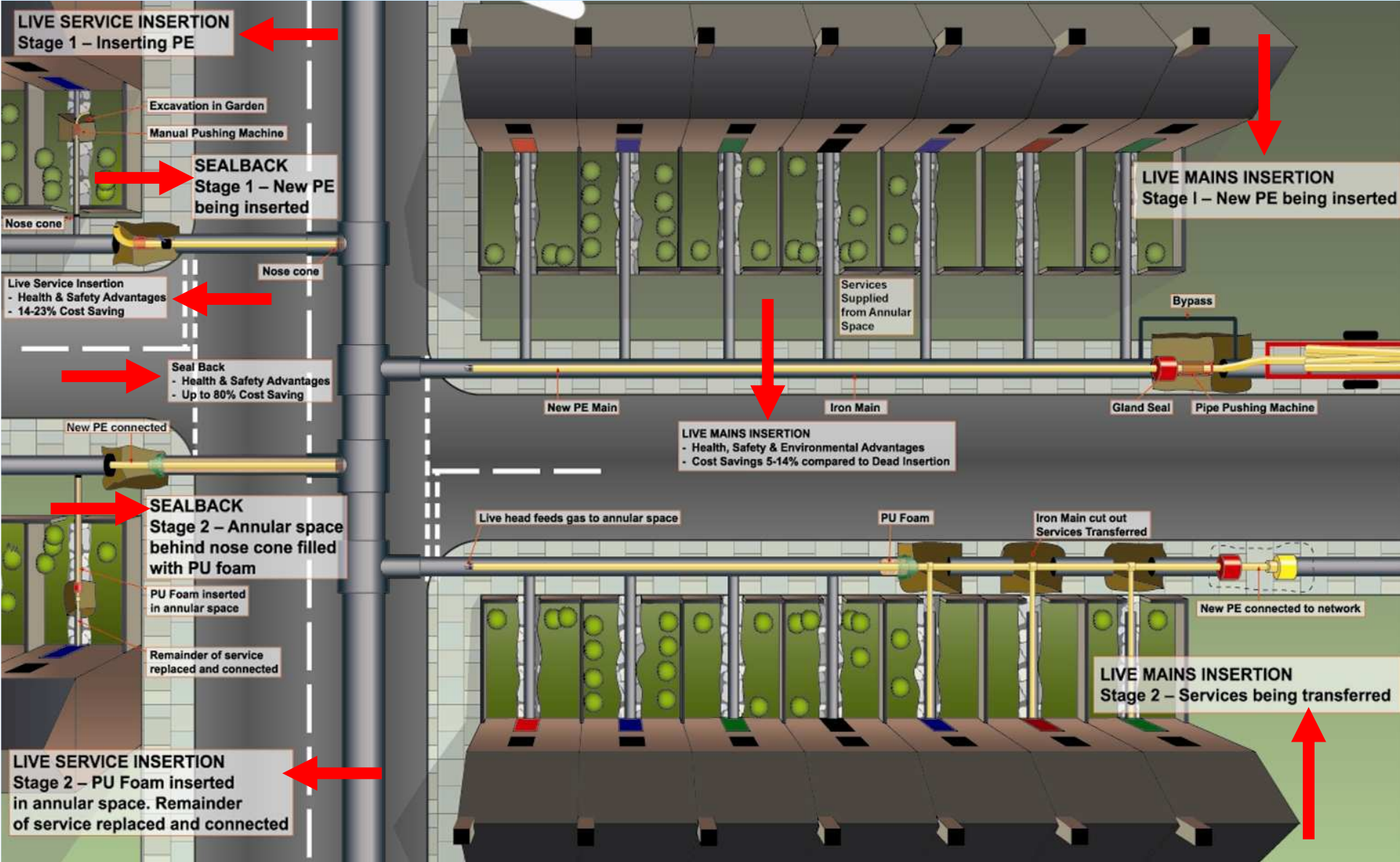
GAS DISTRIBUTION MAINS AND SERVICE REPLACEMENT BY LIVE SLIPLINING TECHNIQUES
