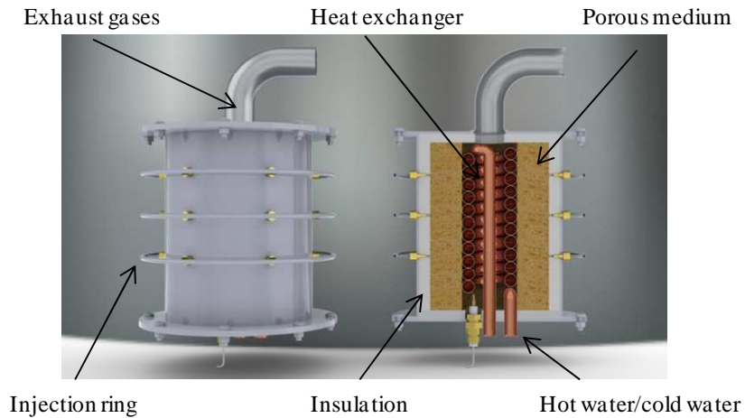
Figure 2 - Basic conception of the compact water heater.
