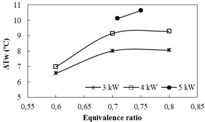
Figure 6 - Increase of the water temperature ( \Delta T_w ) as a function of equivalence ratio.
