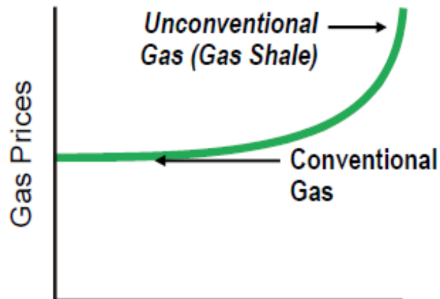
Prior Perception
