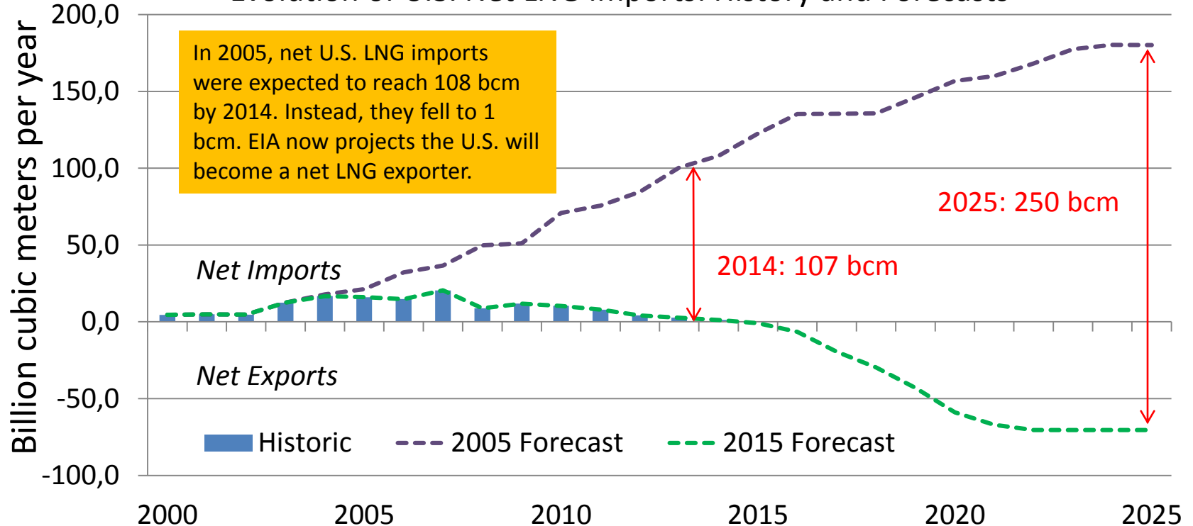
Evolution of U.S. Net LNG Imports: History and Forecasts
