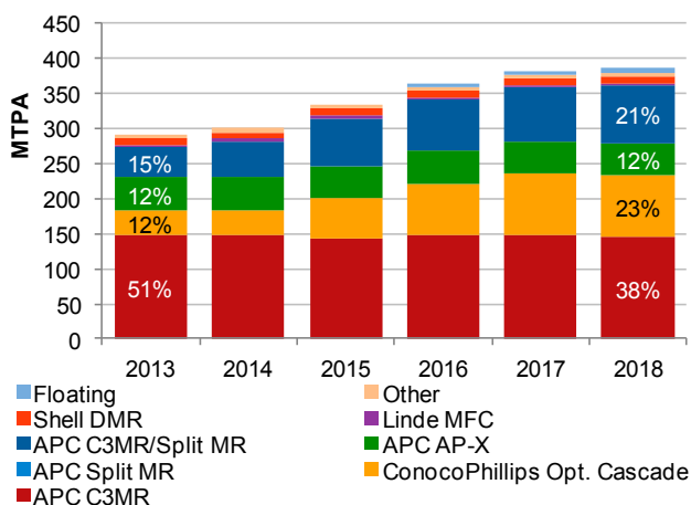
Figure 4.7: Liquefaction Capacity by Type of Technology, 2013-2018
