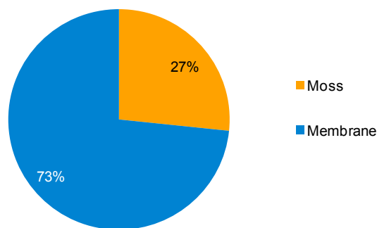
Figure 5.2: Global LNG Fleet by Containment System, end-2013
