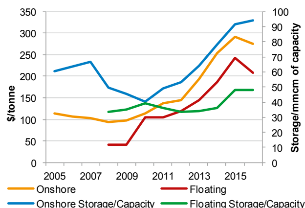
Figure 6.11: Regasification Costs based on Project Start Dates, 2005-2017
