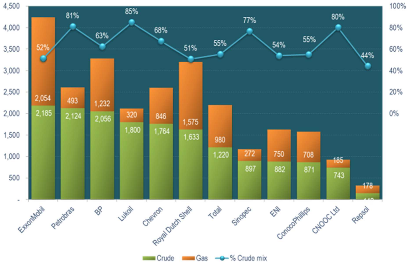
Oil & gas production (thousand bpd)
